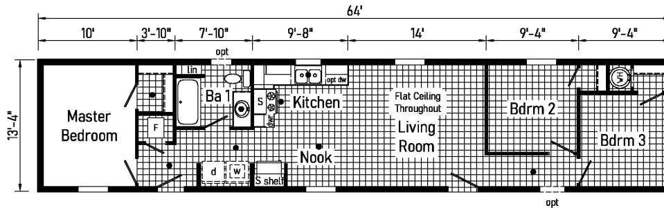
DS1009-P 1464 Approx. 853 Sq. Ft.
