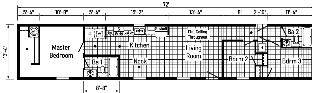
DS1005-P 1472 Approx. 960 Sq. Ft.
