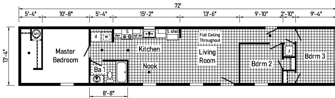
DS1004-P 1472 Approx. 960 Sq. Ft.
