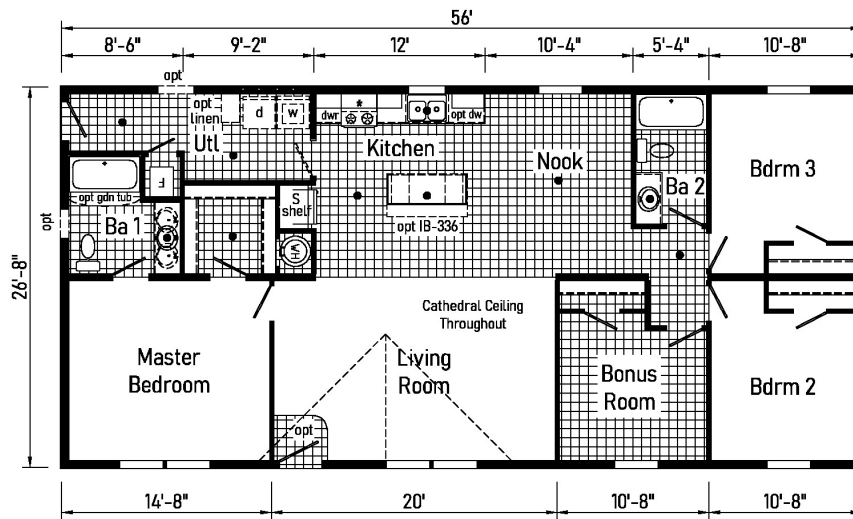
DT1014-P 2856 Approx. 1493 Sq. Ft.
