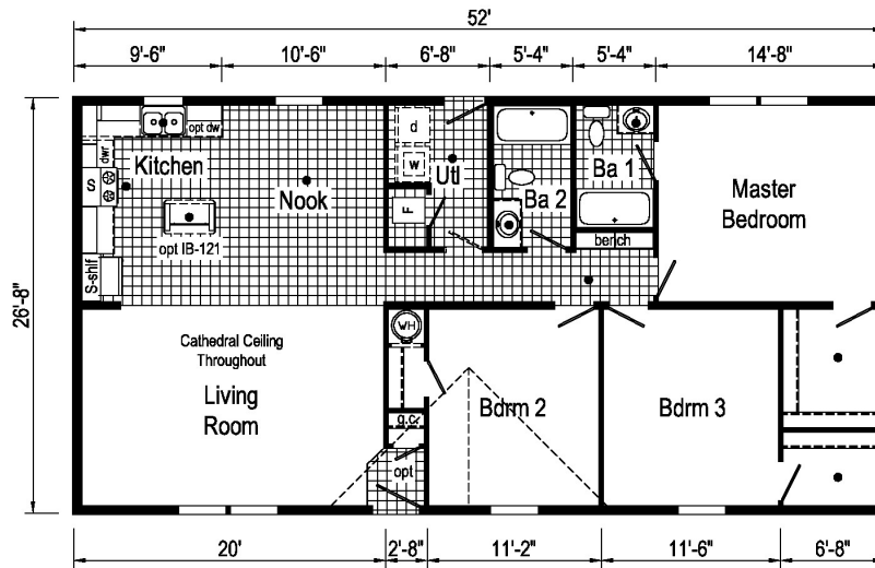
DT1007-P 2852 Approx. 1387 Sq. Ft.
