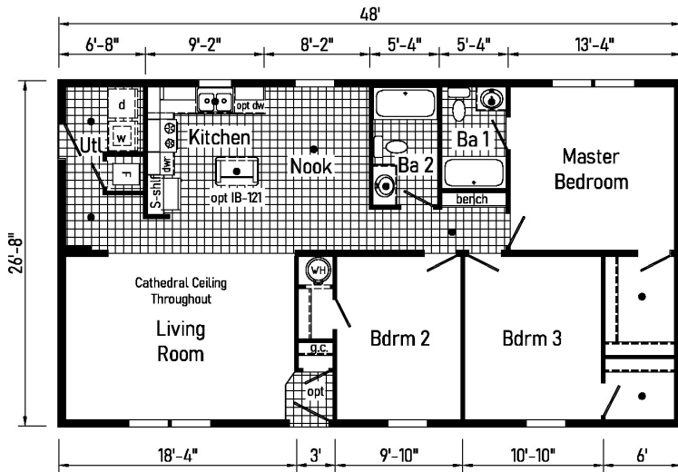
DT1006-P 2848 Approx. 1280 Sq. Ft.
